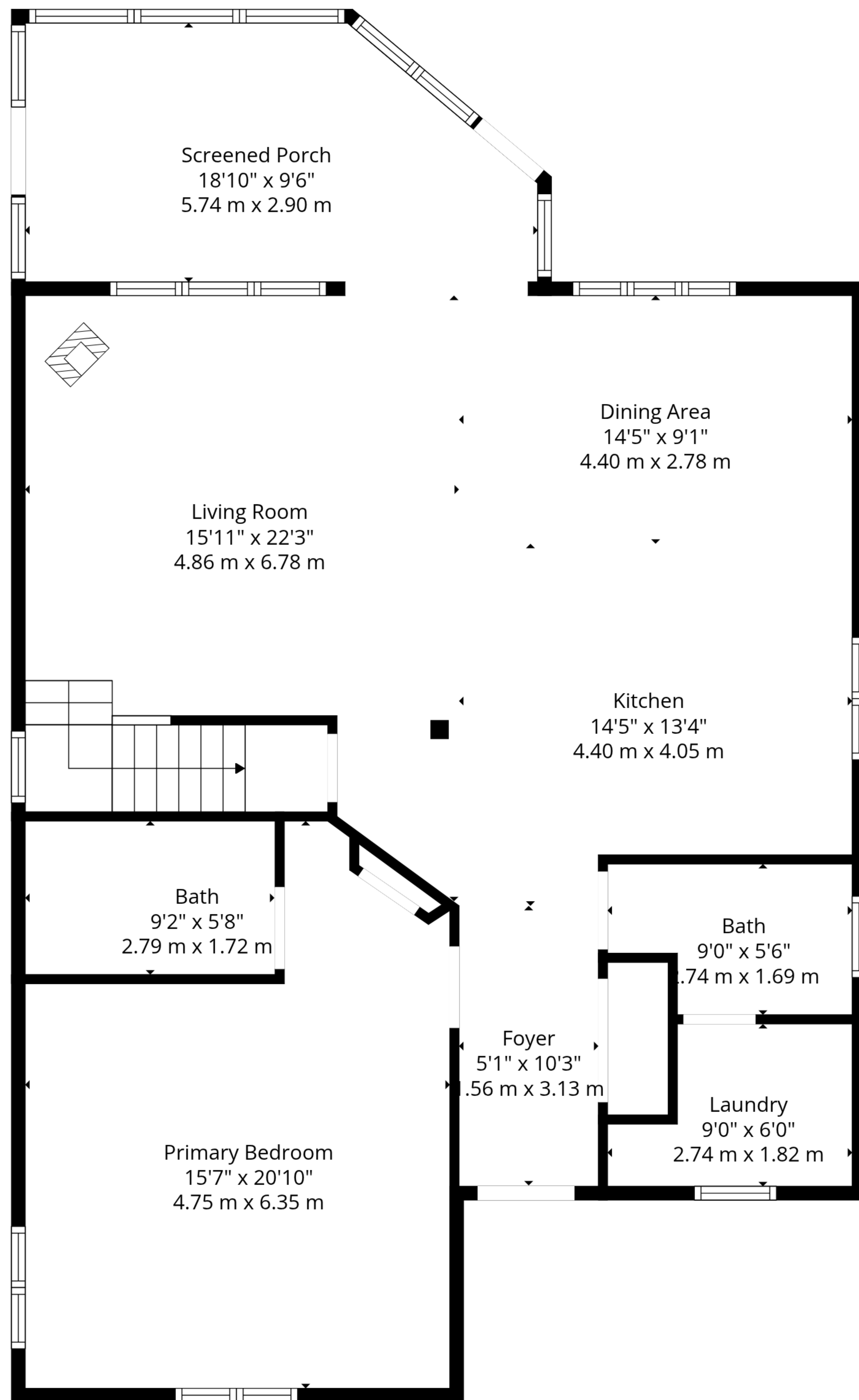
1st Floor
