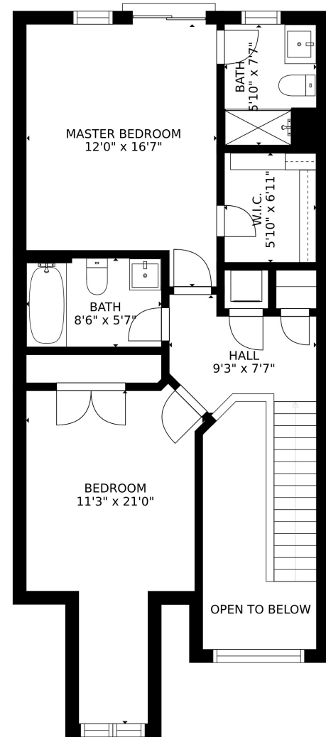
FLOOR 3
