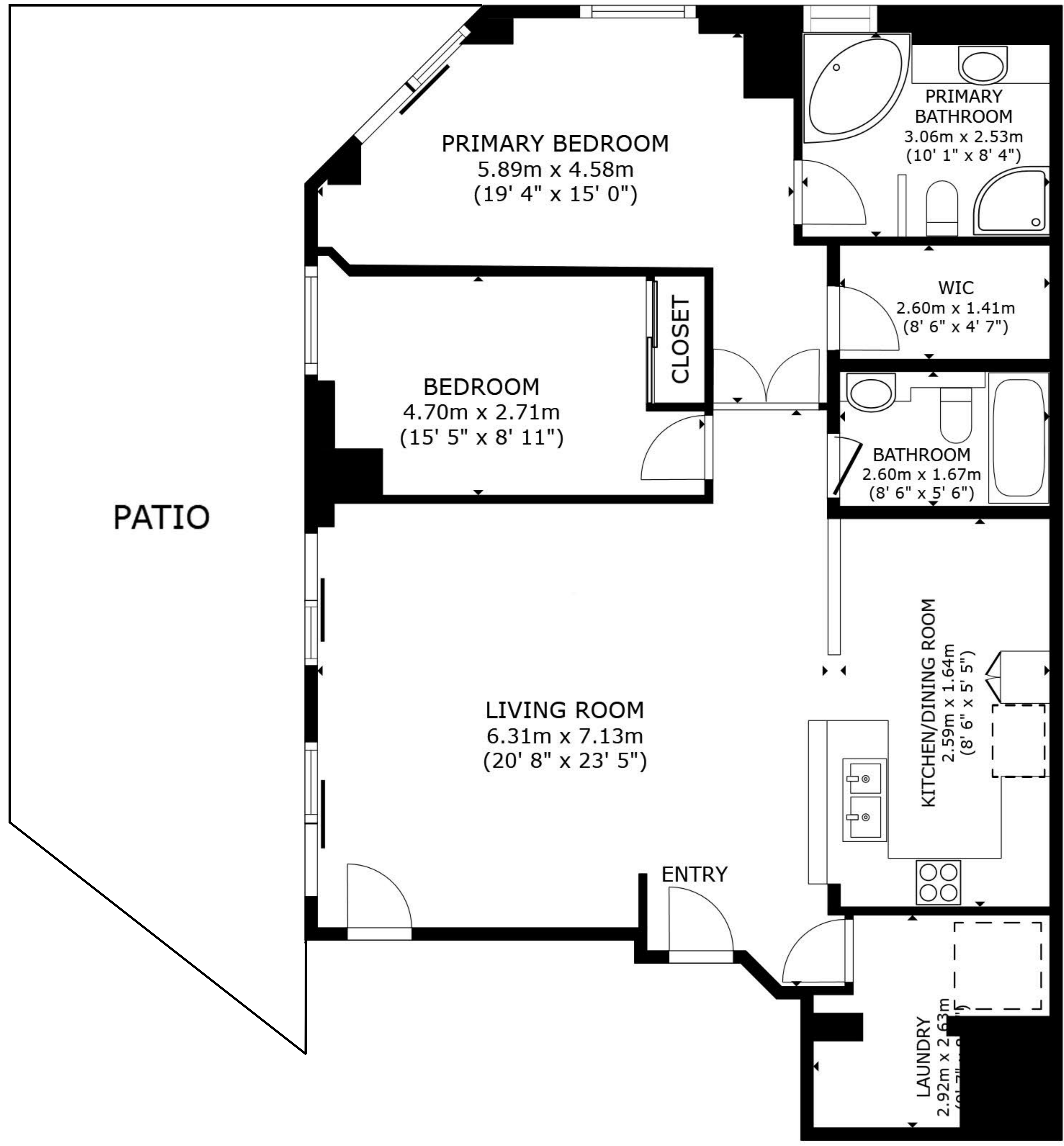
FLOOR PLAN
