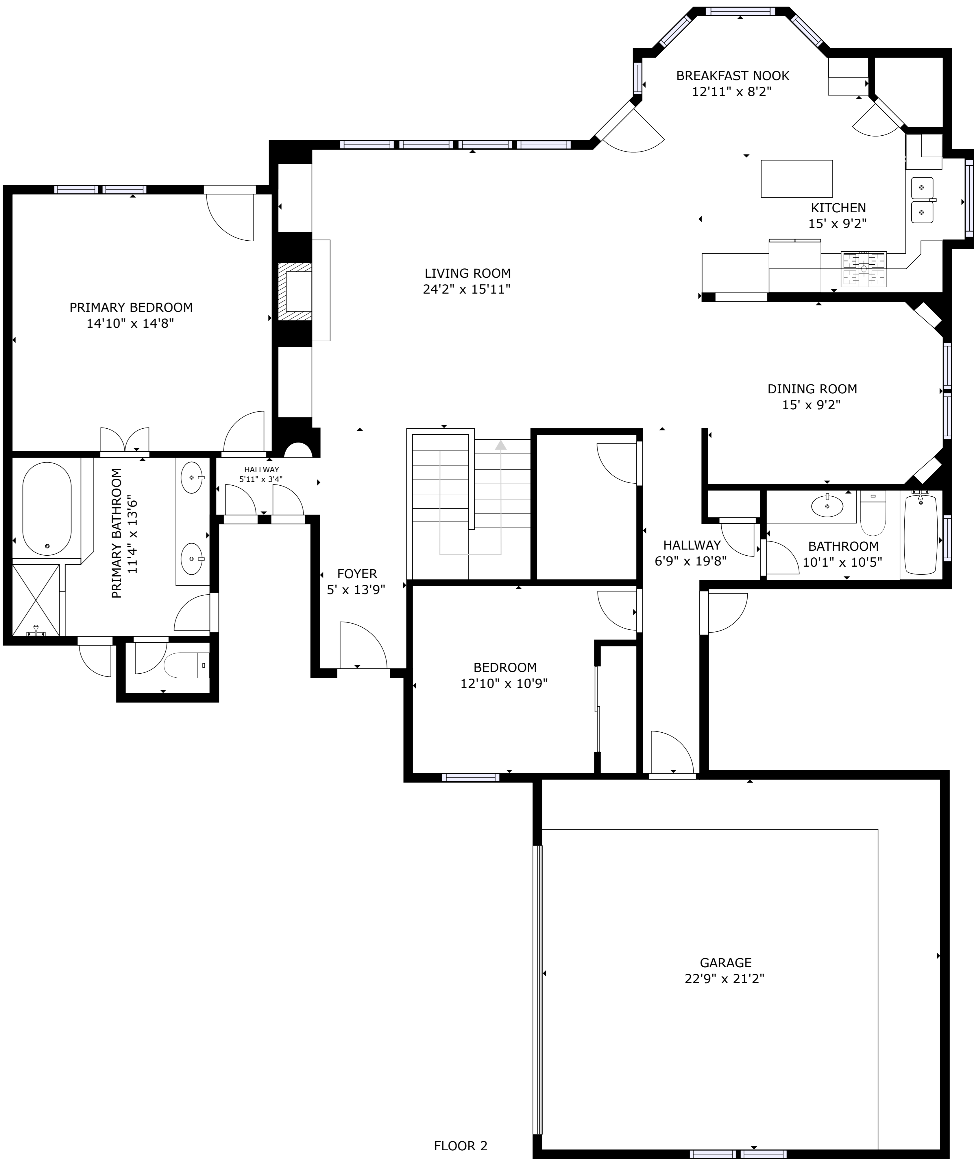
FLOOR 2
