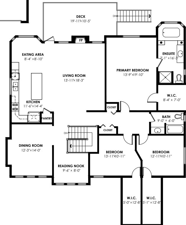
Upper Floor Plan Floor Area: 2038 sq.ft. Ceiling Height: 8'-11"
