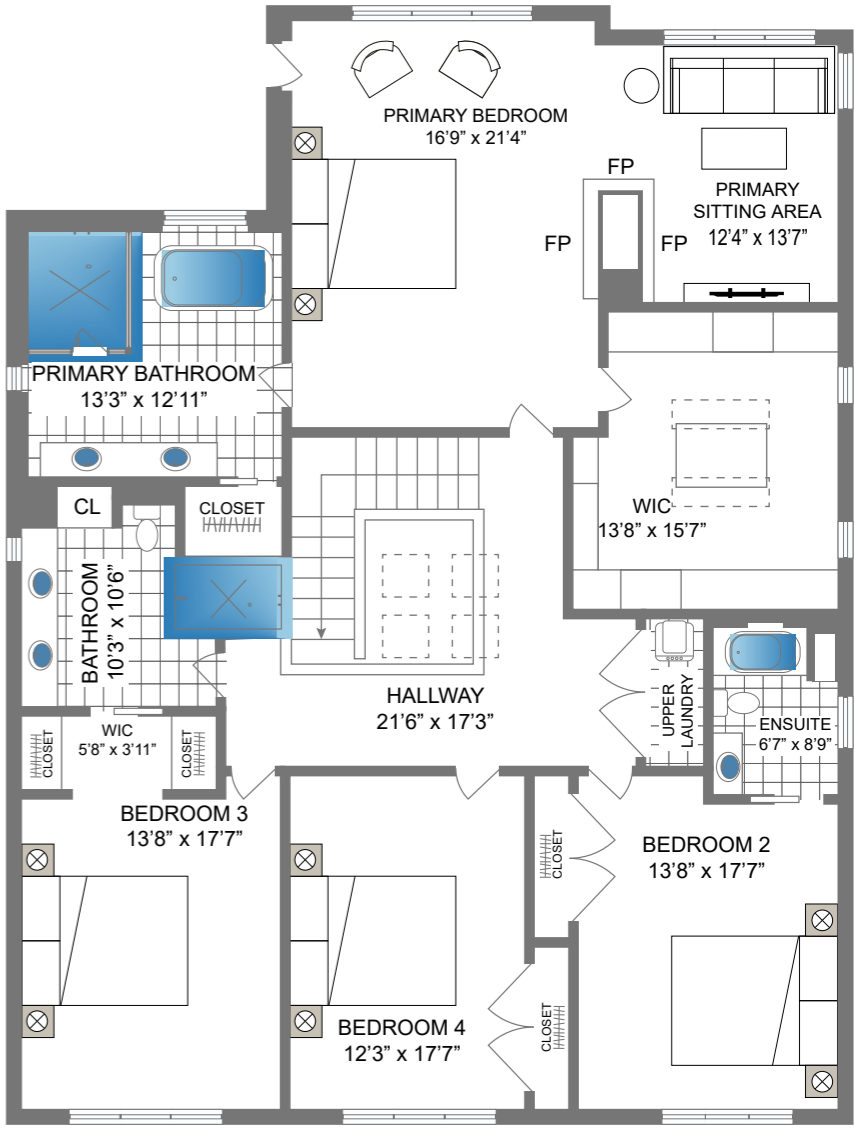
SECOND FLOOR 2,292 SQ. FT.
