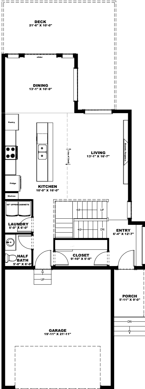
Main Floor
